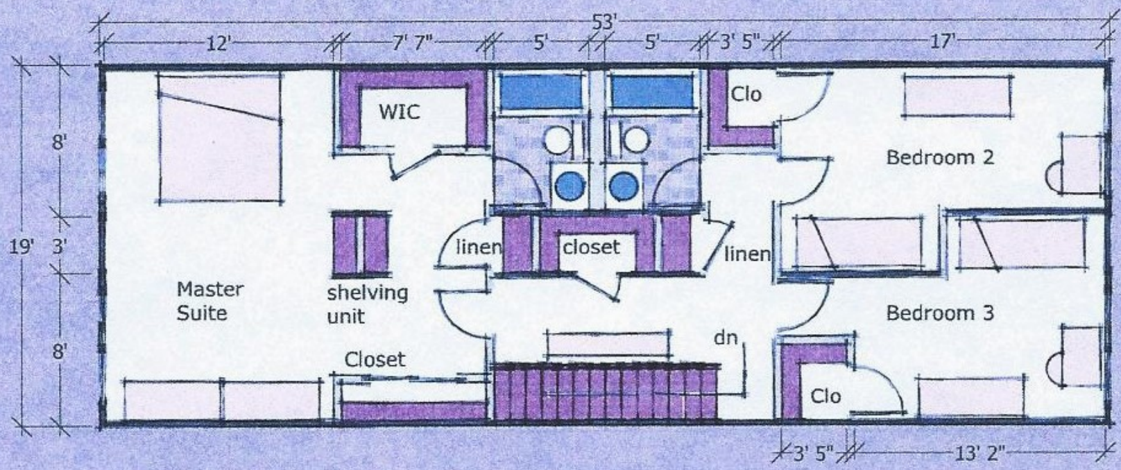
Proposed Second Floor Plan
